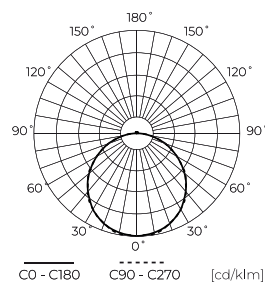
Light distribution
